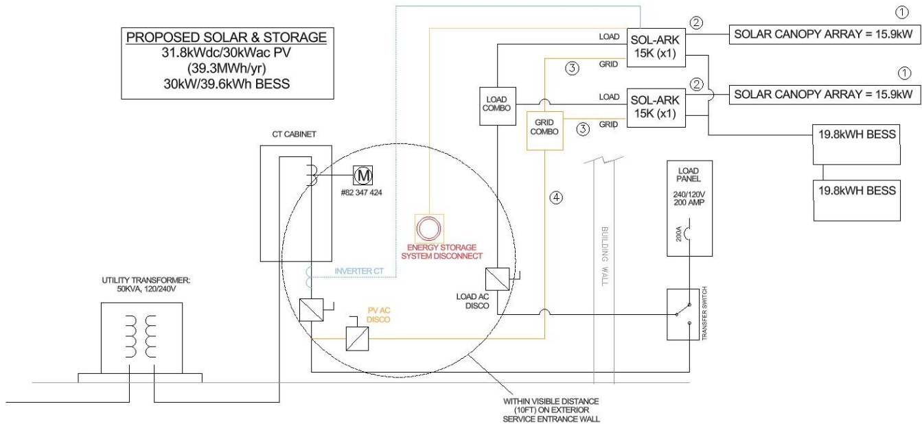
Fig 3.a - Electrical SLD
