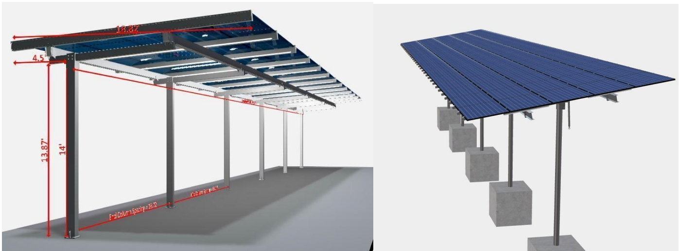
Fig 2.f - Solar Canopy Design based on Infinity Racks (left) and MT Solar (right)
