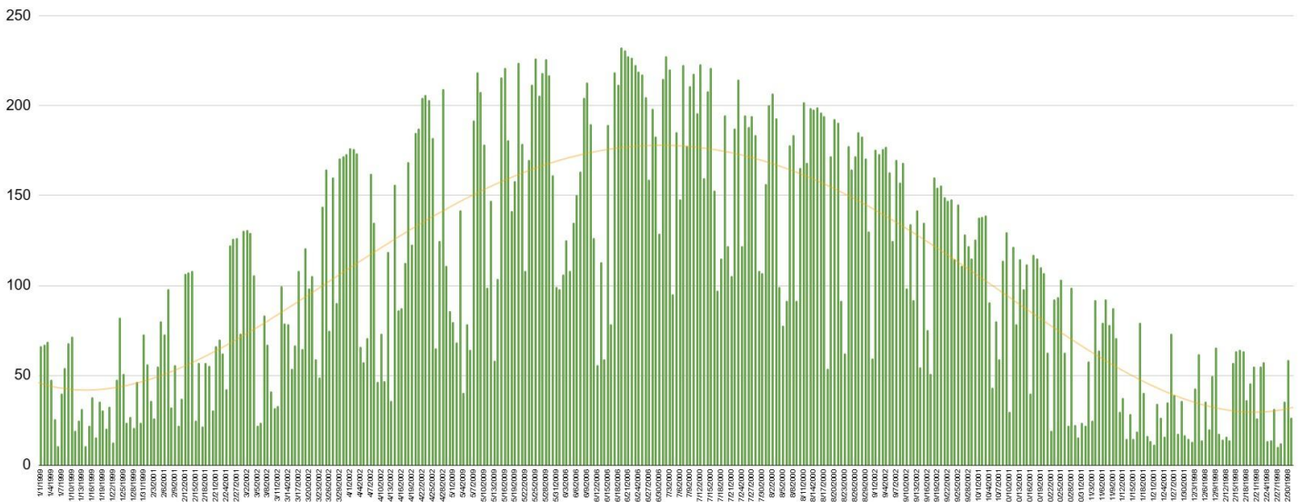
Fig 2.e - Annual kWh/day solar electricity production profile per Helioscope analysis
